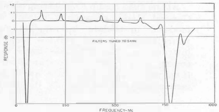
Figure 2. Insertion loss of a Type 874-FR Rejection Filter.
