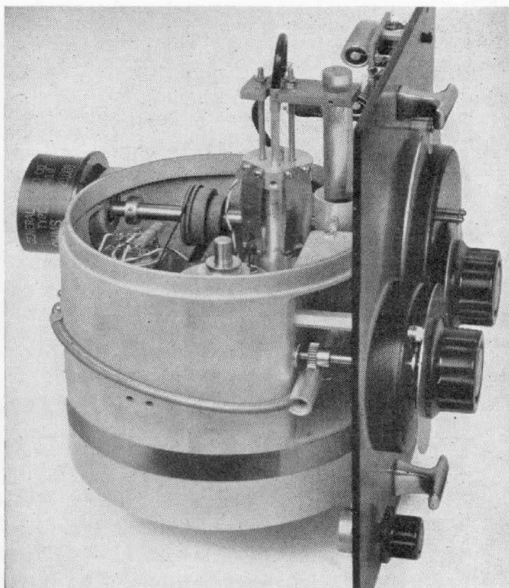
Figure 4. Interior view of the oscillator unit with shield cover removed.
