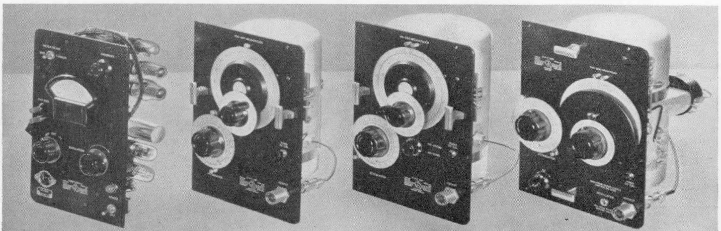
Figure 2. View of the power supply unit and the three oscillator units that make up the Type 1021 series of signal generators. Oscillator units are interchangeable mechanically.
