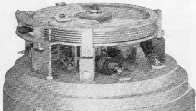
Figure 2. Interior view, showing the location of the two padding capacitors, which are switched into circuit for the 40- to 50-megacycle range extension.
