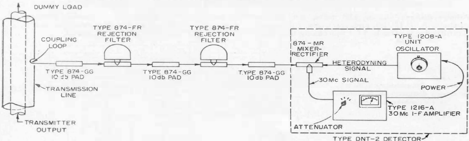
Figure 1. Block diagram of the system for measuring transmitter harmonics. The two rejection filters are isolated by the 10-db pad, which also makes the impedance level 50 ohms.
