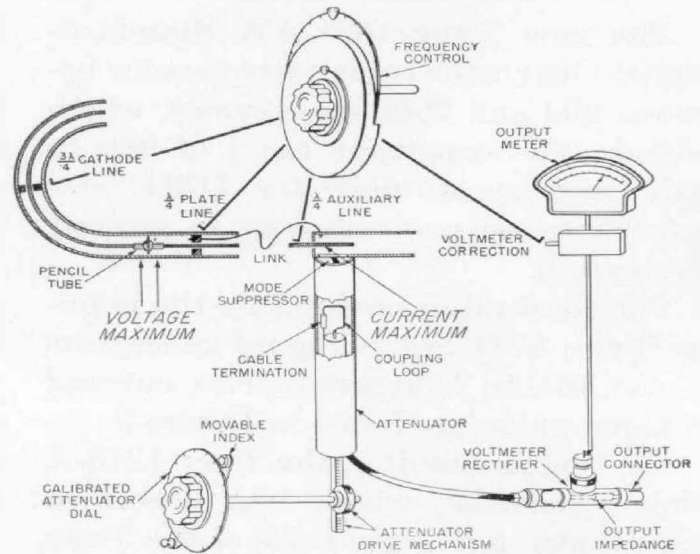
Figure 3. Functional schematic diagram of the new oscillator unit, Type 1021-P4.
