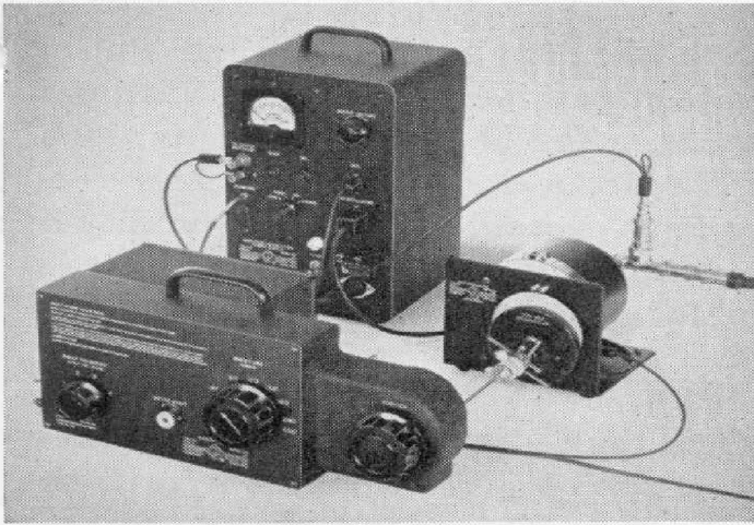
The new Type 1750-A Sweep Drive and Type 1263-A Amplitude-Regulating Power Supply, driving a Type 1209-A Unit Oscillator.
