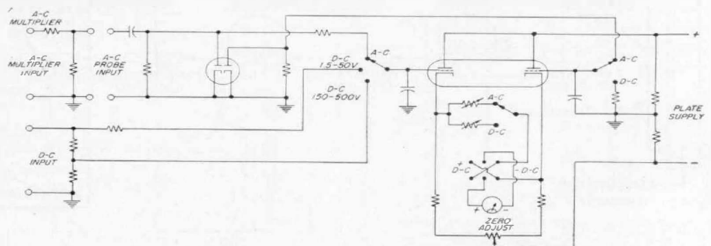
Figure 4. Elementary schematic circuit diagram of the voltmeter.
