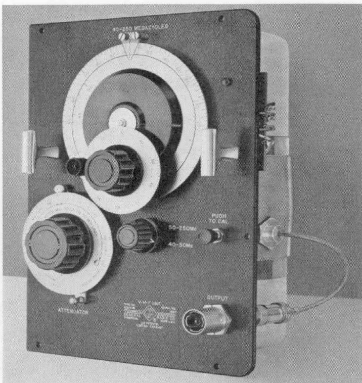
Figure 1. Panel view of the Type 1021-P3B Oscillator Unit.
