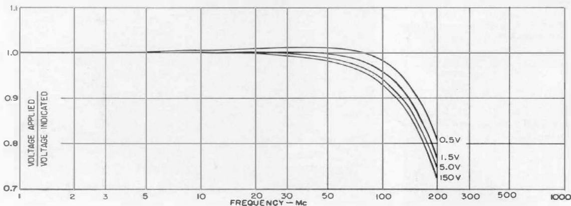
Figure 2. High-frequency correction for the Type 1803-B Vacuum-Tube Voltmeter.
